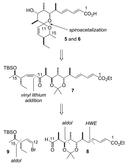
Scheme 1. Retrosynthetic analysis of the pteridic acids leading to key building blocks 8 and 9 .
