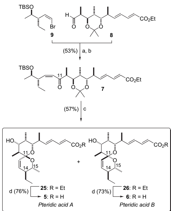
Scheme 4. (a) t BuLi, Et 2 O, –78 °C, 8 , –78 °C; (b) DMP, NaHCO 3 , CH 2 Cl 2 , rt; (c) HF·pyridine, THF/H 2 O (10:1), 0 °C → rt; (d) KOH (aq), EtOH, rt.
