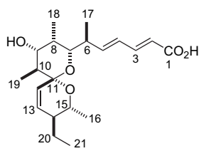
6: Pteridic Acid B
