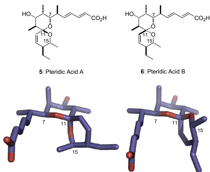
Figure 2. Structures of pteridic acids A and B with calculated minimum energy conformations.
