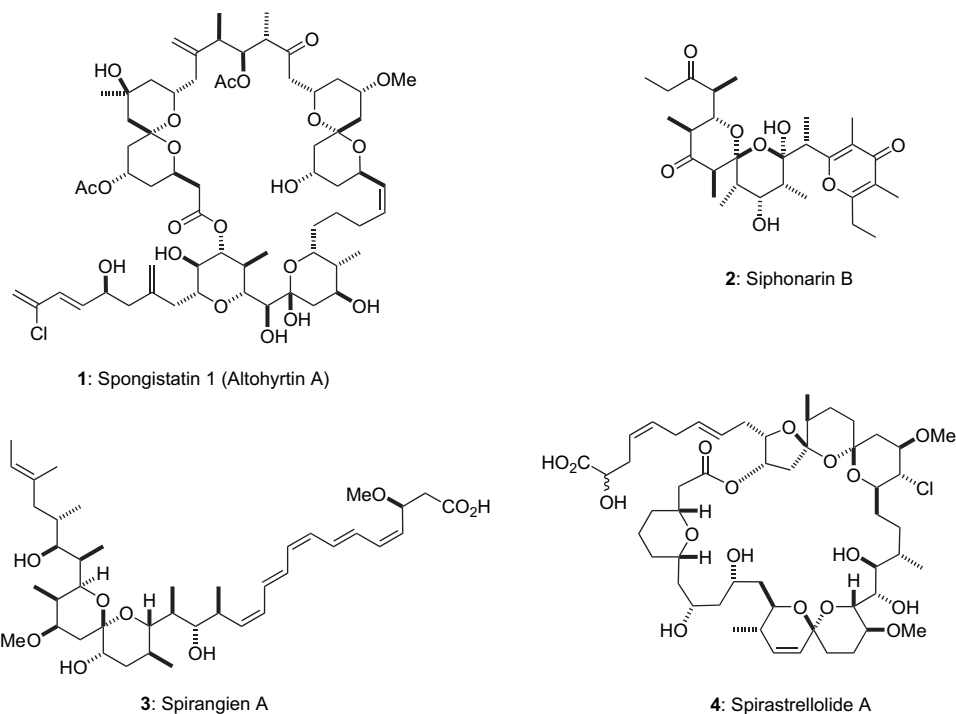
Figure 1. Structures of spiroacetal-containing polyketide natural products.
