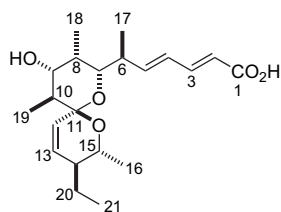
5: Pteridic Acid A
